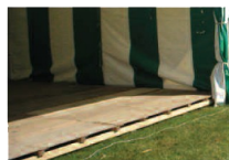
Raised and Levelled Floors
